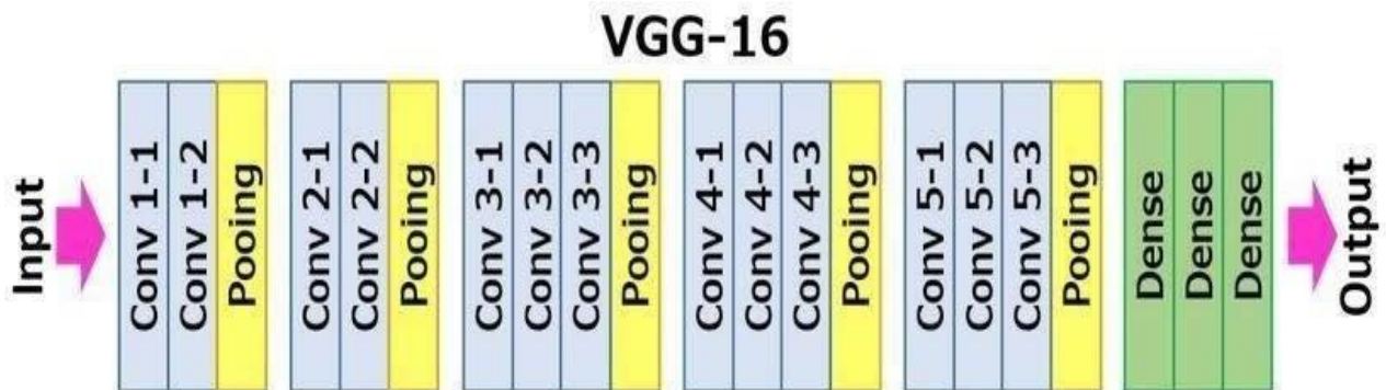
Figure 4: VGG architecture
