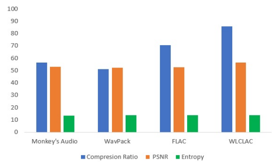
Figure 5: Comparison of the compression and quality parameters for WLCLAC
