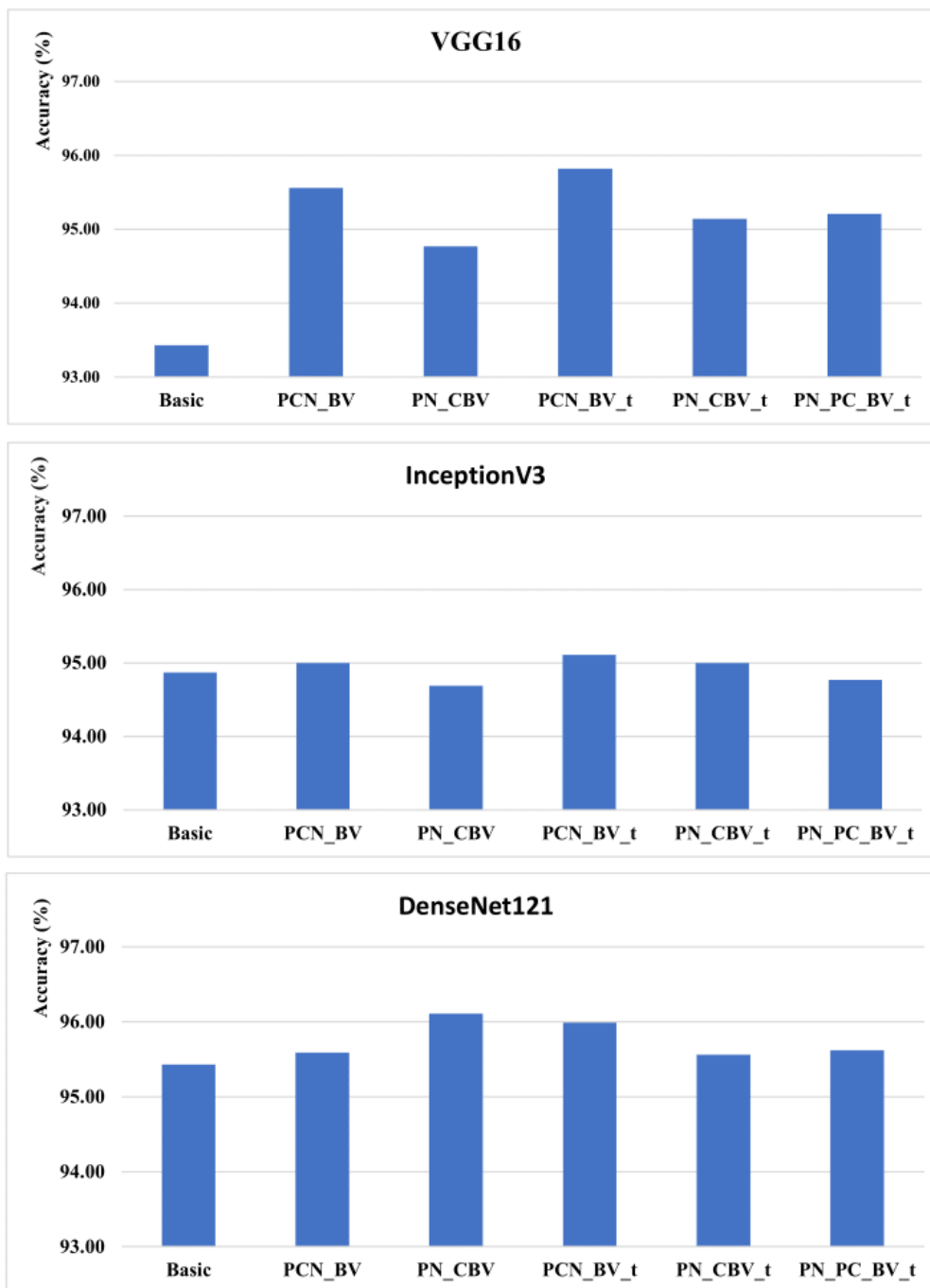
Figure 3: Comparison between transfer learning from ImageNet and transfer learning within the three cascade systems (1)
