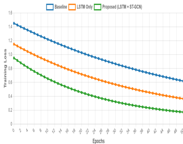
Figure 3: Comparative training loss curves over epochs for baseline, LSTM, and proposed LSTM + ST-GCN models
