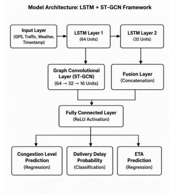
Figure 1: Model architecture LSTM + ST-GCN framework
