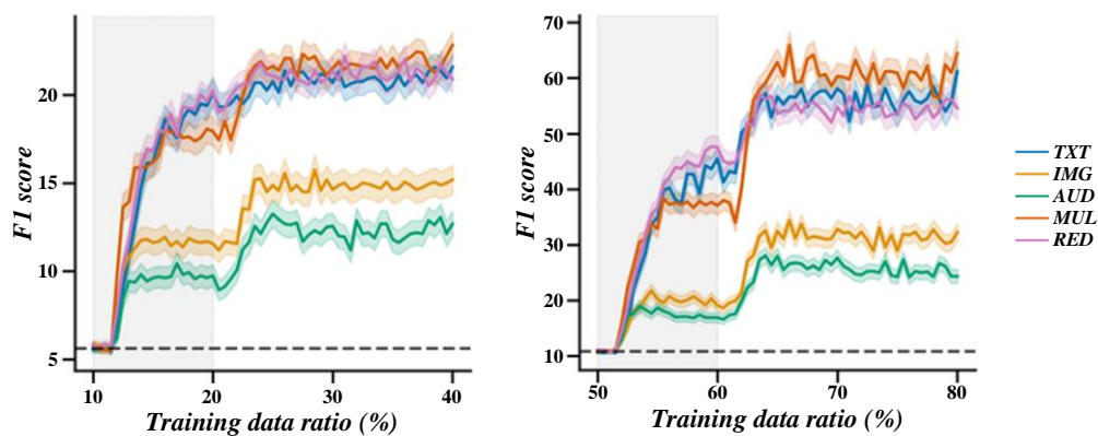
Figure 4: Influence of multimodal characteristic ablation experiment on F1 score
