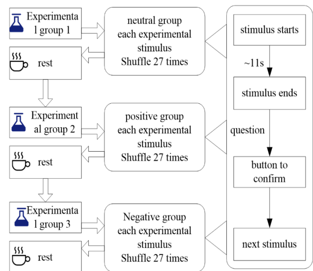
Figure 6: Experimental flow.
