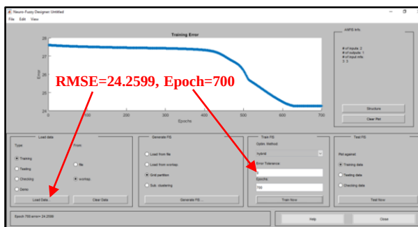
Figure 14: The Epoch error
