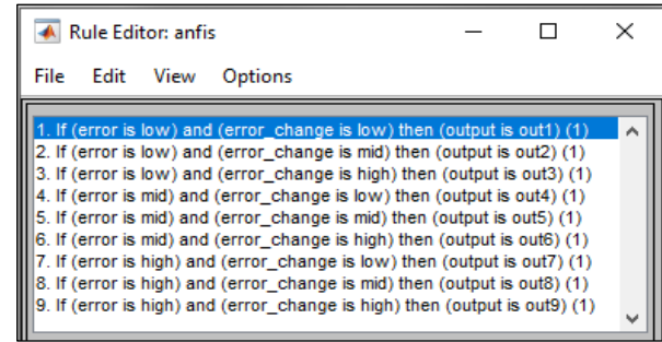
Figure 16: Fuzzy rule bases
