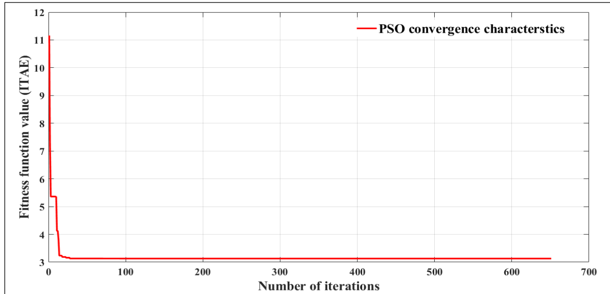
Figure 3: PSO convergence characteristics showing the decrease in the best objective function value (ITAE)
