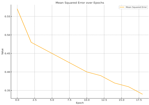
Figure 6: Mean squared error by epoch
