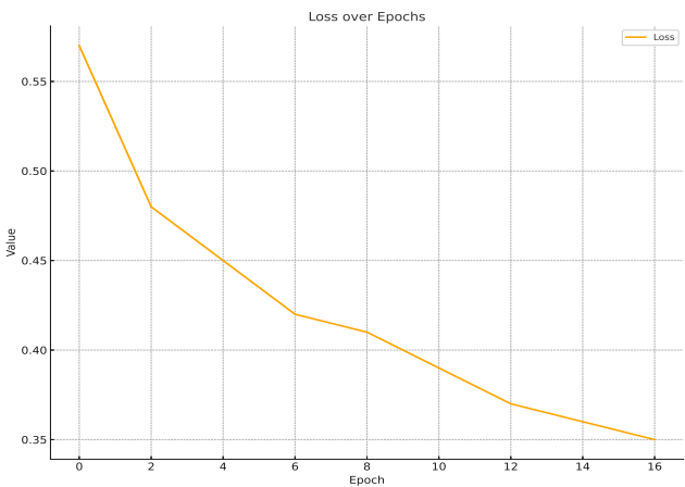
Figure 7: Training and testing losses in 20 epochs
